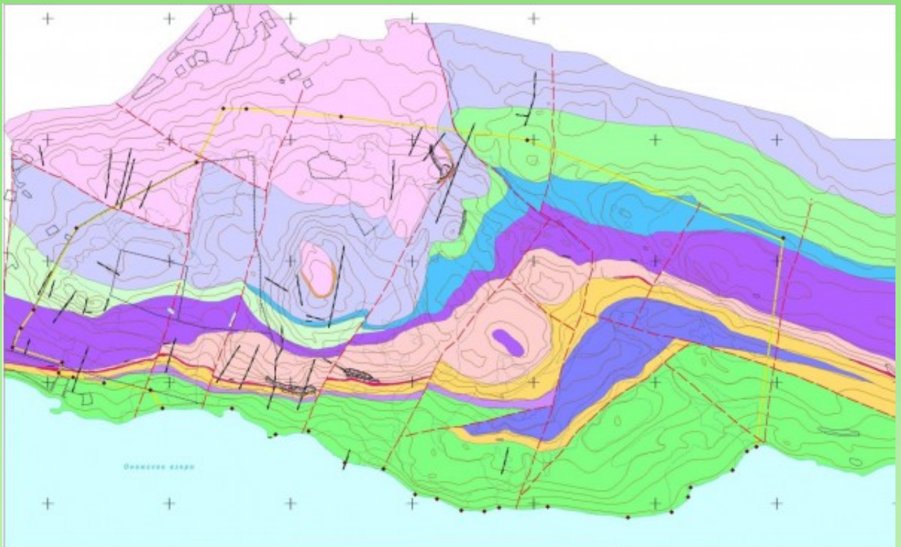
Fig. 4. Geological map of the BG PetrSU. Quaternary sediments.
